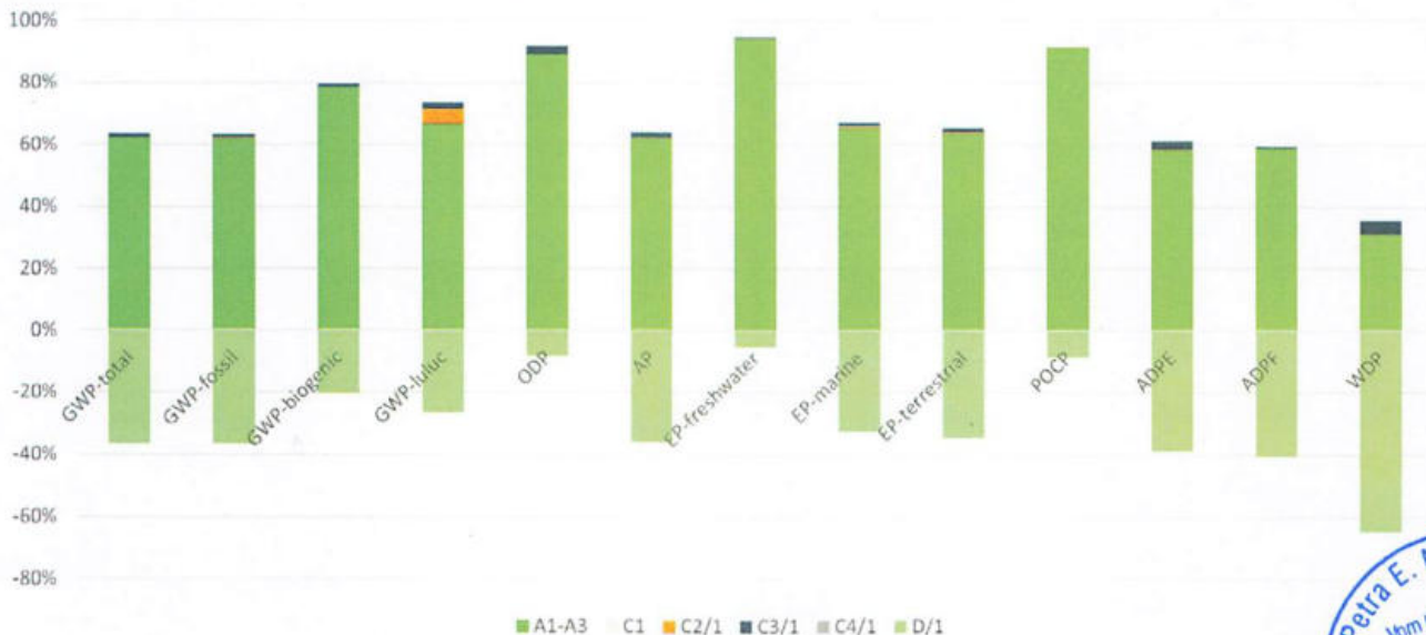
Relative contributions of the various life cycle phases of the blaugelb Triotherm+ Profiles – classic (100 % material recycling)
