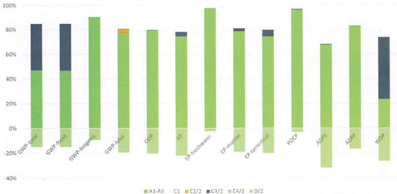
Relative contributions of the various life cycle phases of the blaugelb Insulation Panel MultiPro EPS (100 % energy recovery)
